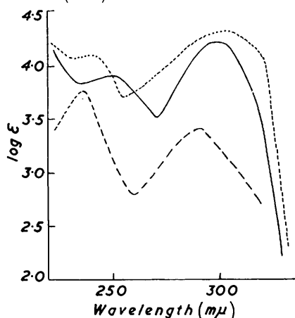
FIG. 1. Ultraviolet spectra of 2-phenylbenzo-1:3-diaza-2-borole (—), 2-phenylbenzimidazole (· · ·) and o -phenylenediamine (---).
